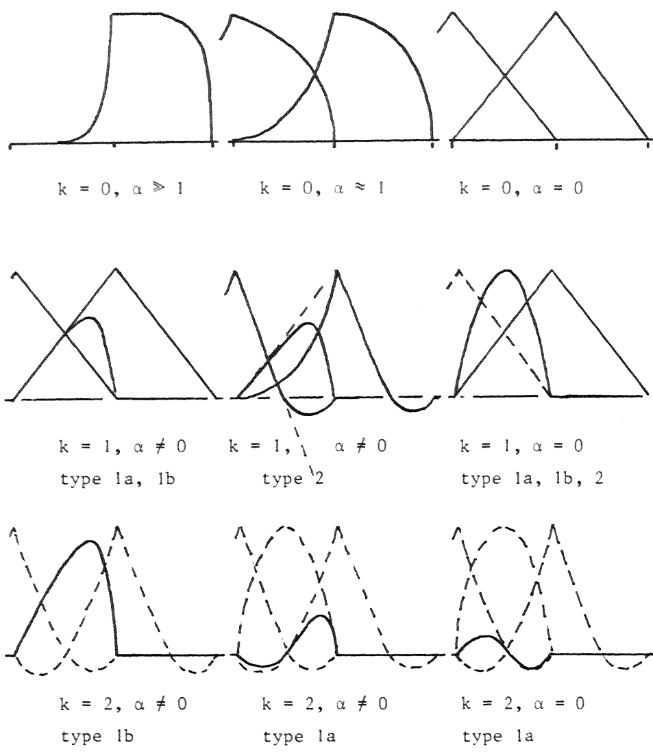
Fig. 2. Several basis functions in E_k^h , k = 0, 1, 2 .
