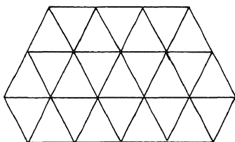
T_h in \Omega \subset \mathbb{R}^2
